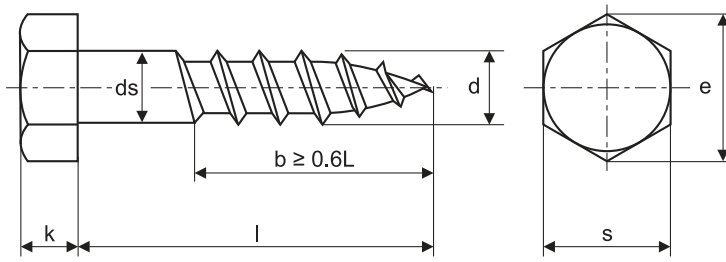
DIN 571 Dimensions of coach screws
